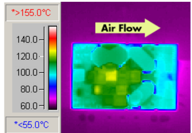
Figure 12: Thermal plot of converter at 17 amp load current with 55°C air flowing at the rate of 200 LFM. Air is flowing across the converter from input to output (48V input).
