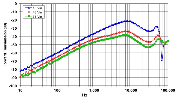
Figure 24: Magnitude of incremental forward transmission ( FT = V_{out}/V_{in} ) for minimum, nominal, and maximum input voltage at full rated power.
