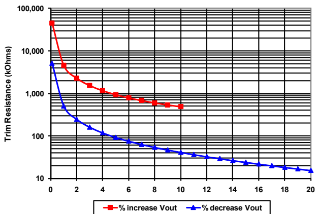
Figure C: Trim Graph
