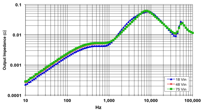
Figure 23: Magnitude of incremental output impedance ( Z_{out} = v_{out}/i_{out} ) for minimum, nominal, and maximum input voltage at full rated power.
