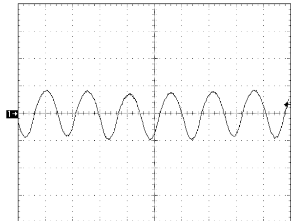
Figure 18: Input Terminal Ripple Current, i_c , at full rated output current and nominal input voltage with 10\mu H source impedance and 47\mu F electrolytic capacitor (200 mA/div). See Figure 17.
