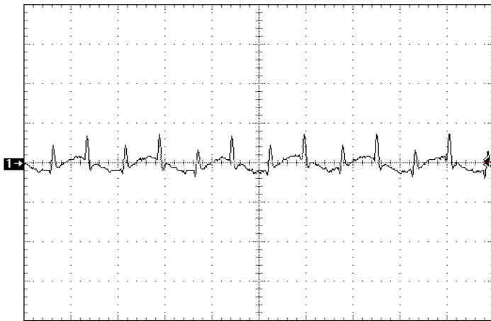
Figure 19: Input reflected ripple current, i_p , through a 10\ \mu\text{H} source inductor at nominal input voltage and rated load current (20 mA/div). See Figure 17.
