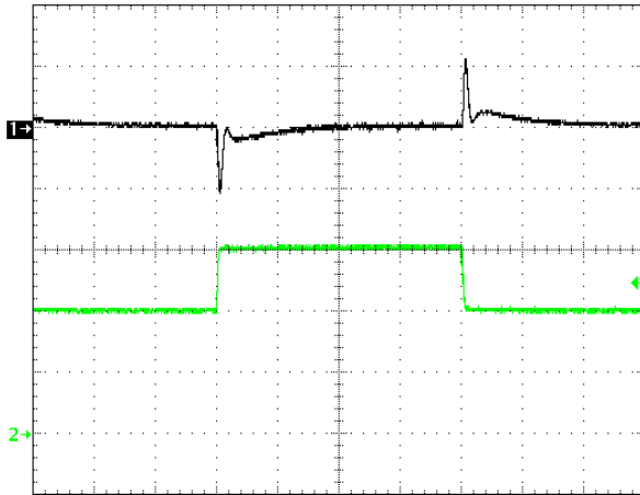
Figure 15: Output voltage response to step-change in load current (50%-75%-50% of I_{out(max)} ); dI/dt = 0.1A/\mu s . Load cap: 10\mu F , 100\text{ m}\Omega ESR tantalum cap and 1\mu F ceramic cap. Ch 1: Vout (200mV/div), Ch 2: I_{out} (5A/div).
