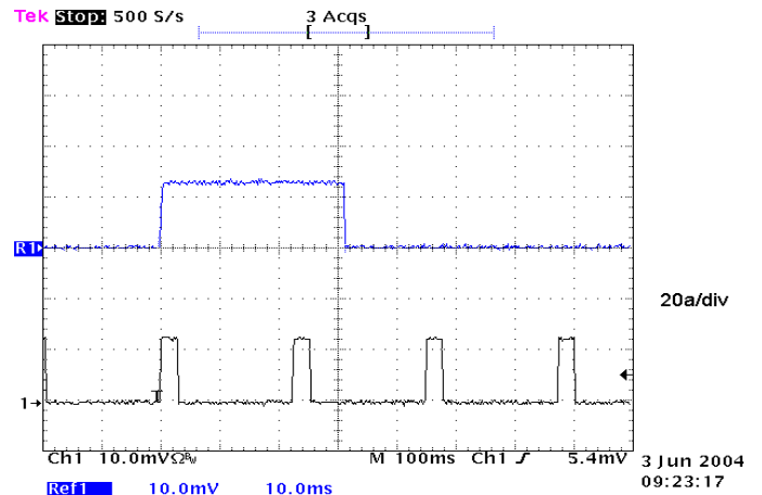
Figure 22: Load current (20A/div) as a function of time when the converter attempts to turn on into a 10 mW short circuit. Top trace (10ms/div) is an expansion of the on-time portion of the bottom trace.
