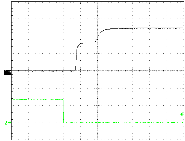
Figure 14: Turn-on transient at zero load (5 ms/div). Ch 1: Vout (2V/div). Ch 2: ON/OFF input (5V/div).
