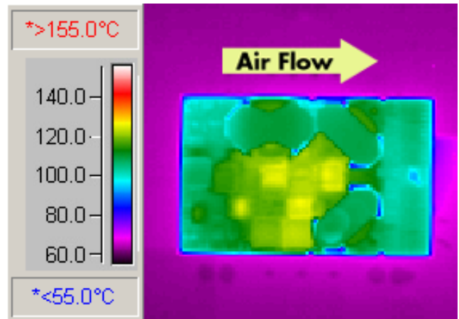
Figure 10: Thermal plot of converter at 19 amp load current with 55°C air flowing at the rate of 200 LFM. Air is flowing across the converter from input to output (24V input).
