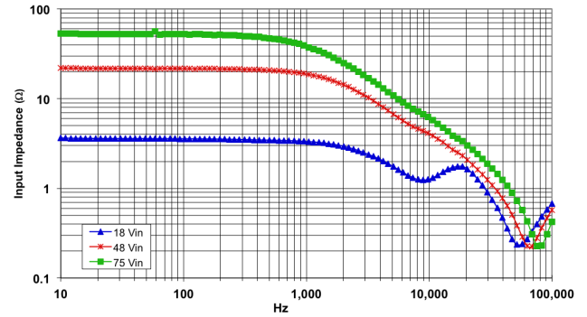
Figure 26: Magnitude of incremental input impedance ( Z_{in} = V_{in}/i_{in} ) for minimum, nominal, and maximum input voltage at full rated power.
