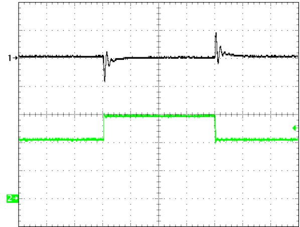
Figure 16: Output voltage response to step-change in load current (50%-75%-50% of I_{out(max)} ); dI/dt = 5A/\mu s . Load cap: 470\mu F , 30\text{ m}\Omega ESR tantalum cap and 1\mu F ceramic cap. Ch 1: Vout (200mV/div), Ch 2: I_{out} (5A/div).
